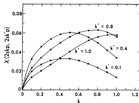
FIG. 3. Beryllium free-free matrix elements.
